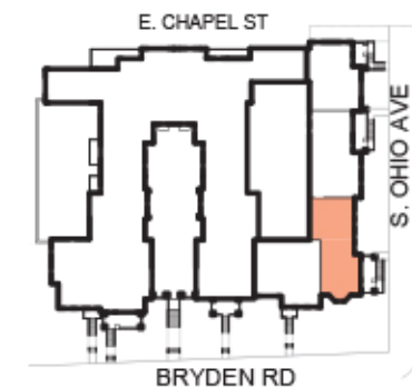
UNIT 11 - SECOND FLOOR PLAN
