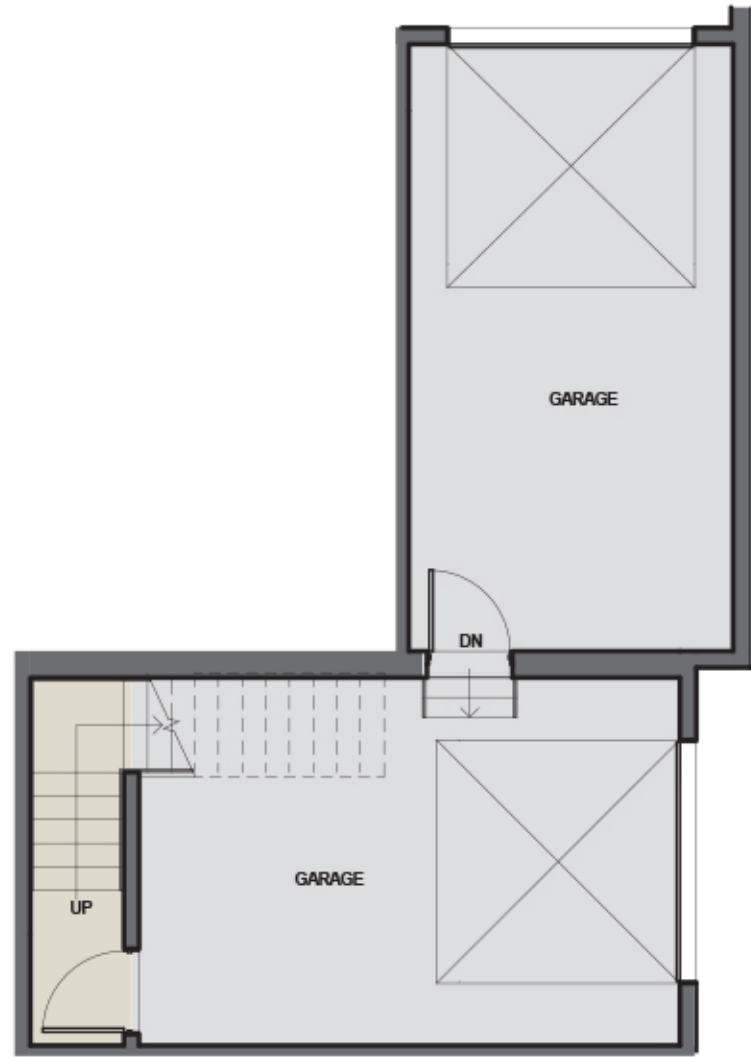
UNIT 7 - BASEMENT PLAN
